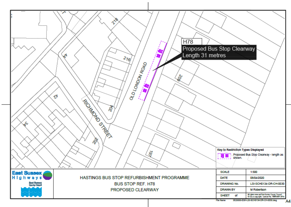
Fig 2: Plan showing the proposed Clearway markings on Old London Road.
